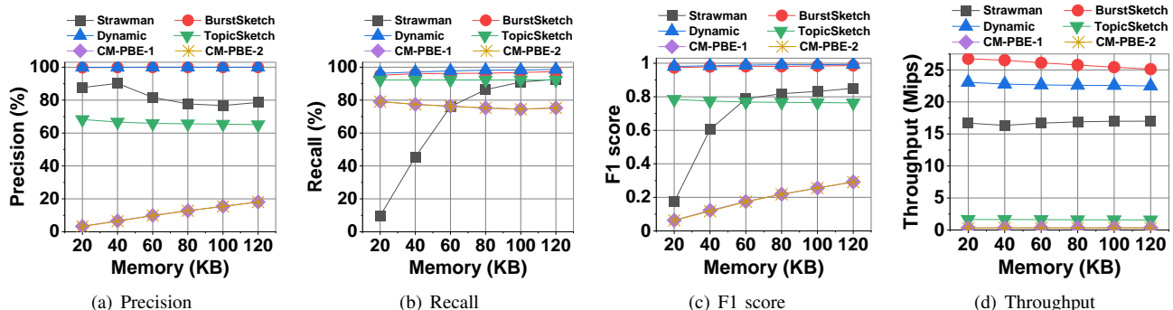
Fig. 7: Experiments on Network datasets.
