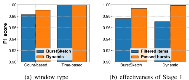
Fig. 9: Analyses on BurstSketch and the optimization, including window type and the effectiveness of Stage 1.
