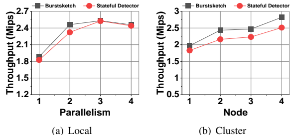
Fig. 10: Comparison between BurstSketch and Stateful Detector on Apache Flink
