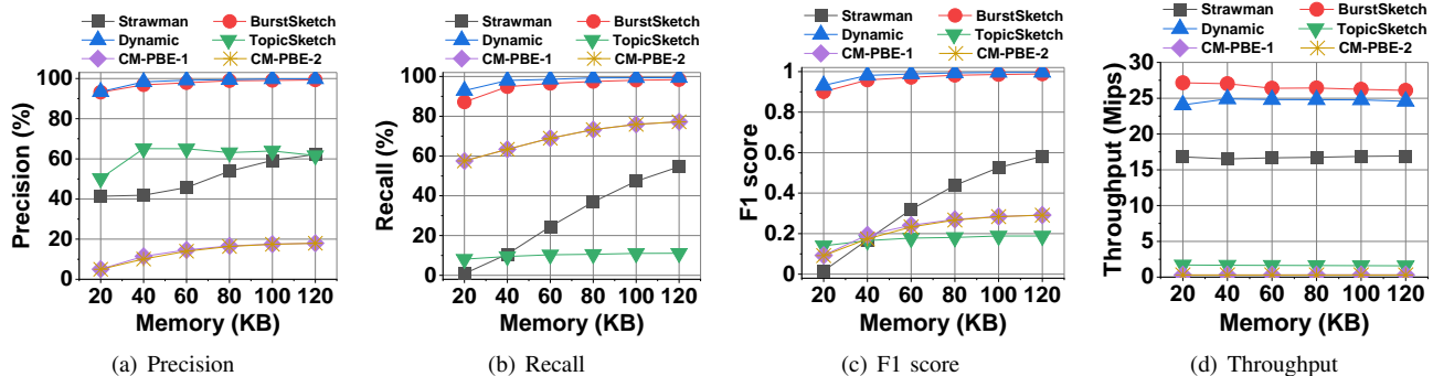
Fig. 6: Experiments on Web Page datasets.
