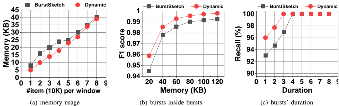
Fig. 8: Analyses on BurstSketch and the optimization, including memory usage for different data stream speed, detecting burst inside burst, and performance under different bursts' duration.
