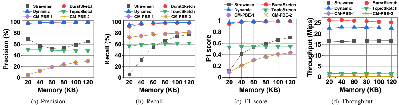
Fig. 5: Experiments on CAIDA datasets.
